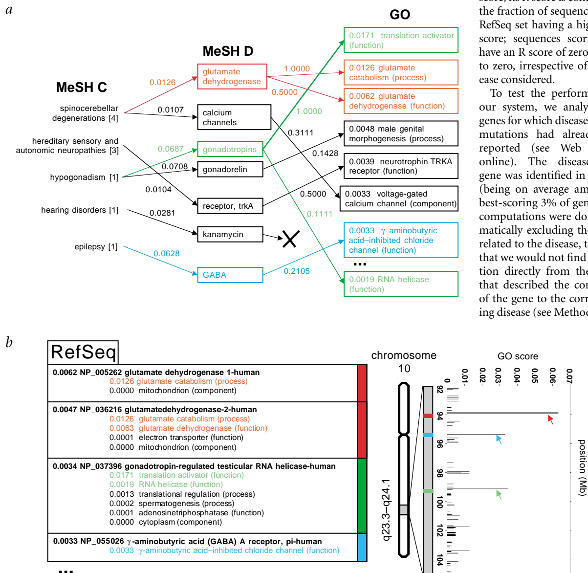
Fig. 2 Example of the analysis of 'spinocerebellar ataxia-8, infantile, with sensory neuropathy'. The red/blue/green colored boxes indicate different protein functions. a , Spinocerebellar ataxia-8 was linked to a number of medical terms (left column, MeSH C terms; the number in brackets indicates the number of papers in which the terms were present). Using the previously derived relations, we could evaluate the more-related functional terms (right column, GO terms). For example, the strength of the association of the pair (hypogonadism, translation activator) is defined by a path through the MeSH D term 'gonadotropins', which gives a value of 0.0687 \times 1.0000 = 0.0687 (see Methods). Taking into account that the MeSH C term 'hypogonadism' was associated with one of four papers describing the disease, the corresponding value for the weighted association \mu_{T,w} (hypogonadism, translation activator) is 0.0687 \times 1/4 = 0.0171 . As this value is the maximum \mu_{T,w} pointing to 'translation activator' from any MeSH C, the corresponding GO term 'translation activator' receives a score \mu_{T,w} (translation activator) of 0.0171. b , Regions of homology to the 10,000 RefSeq sequences were searched on a region of chromosome 10 (positions 92–105 Mb) where the disease had been mapped. The four sequences that best match the disease, according to their annotations (GO terms, indicated as in a ) and for which homology was found, are shown on the left. The first two sequences are homologous and therefore point to the same region. The graph on the right indicates the GO score of the matching sequence versus the position in the hit in the region. The color (red/green/blue) to the right of the sequence annotation box indicates the region of the match. The three hits pointed in the graph by the arrows stand well above the rest: one of them is likely to correspond to the gene underlying this disease.
